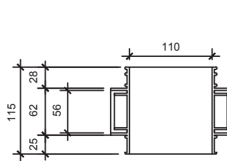
4" Pipe Sleeve With Inlet
