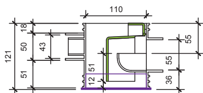
Side Flow Trap Body
