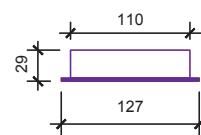
4" End Cap
