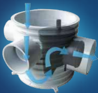
SIDE FLOW CONCEALED FLOOR TRAP
