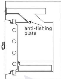
CROSS-SECTION - FRONT DRAWER TRAP
