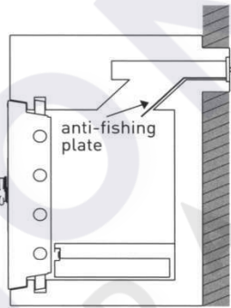
CROSS-SECTION - BACK DRAWER TRAP
