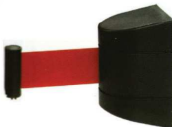
OKWMRB-201 LENGTH OF BELT : 2 METER HEAD SIZE : 75mm(W) x 100mm(D) x 140mm(H)
