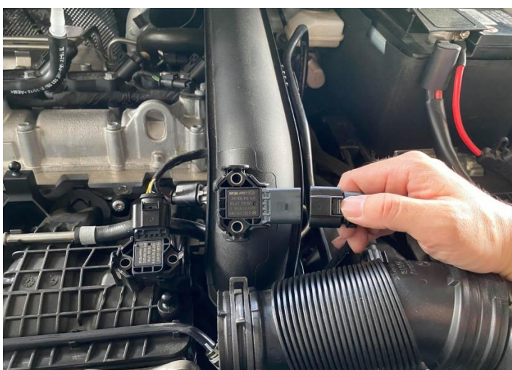
Figure 5: 斷開原廠渦輪管上方感應器接頭
