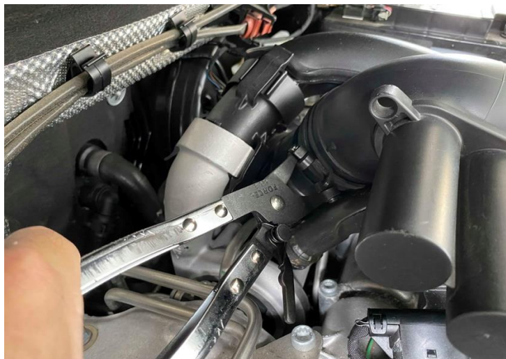
Figure 1: 鬆開渦輪端進氣管管束
