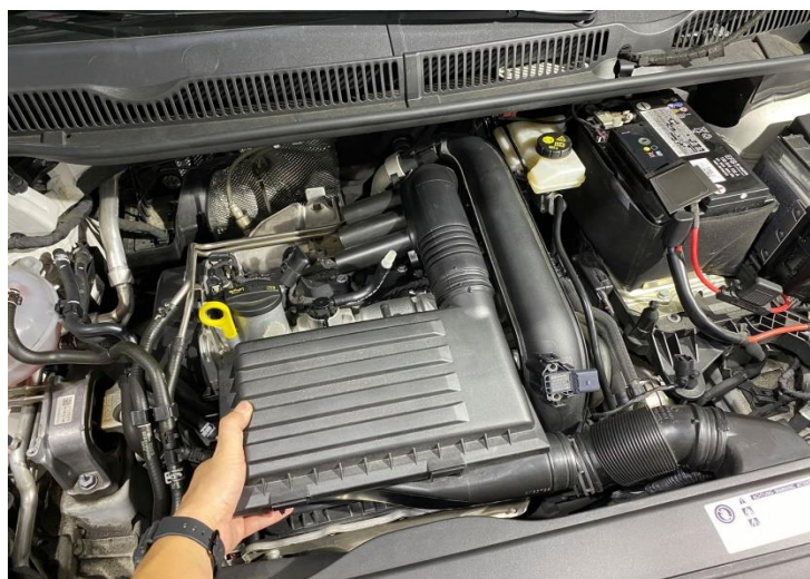
Figure 15: 回復安裝集氣箱
