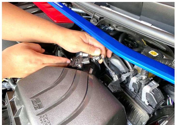
Figure 6: Disconnect the MAF sensor plug.
