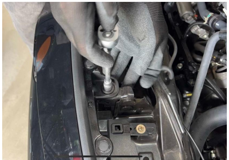
Figure 18: Remove the m6 screw.
