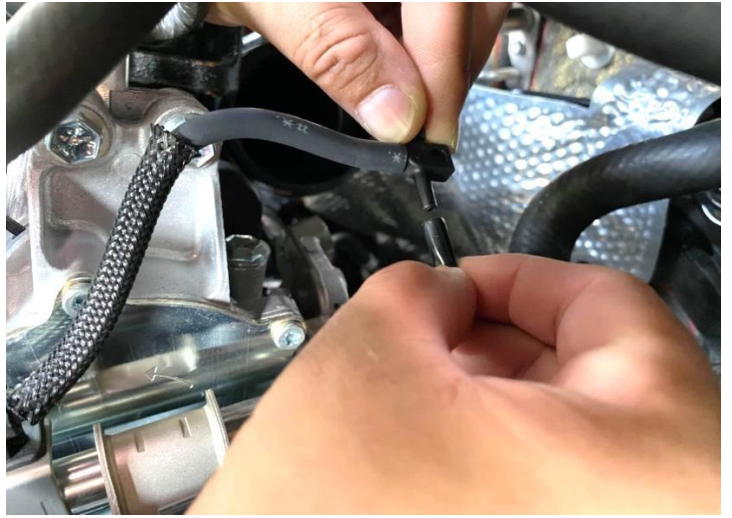
Figure 10: 4mm rubber cap to plug the T-Piece.
