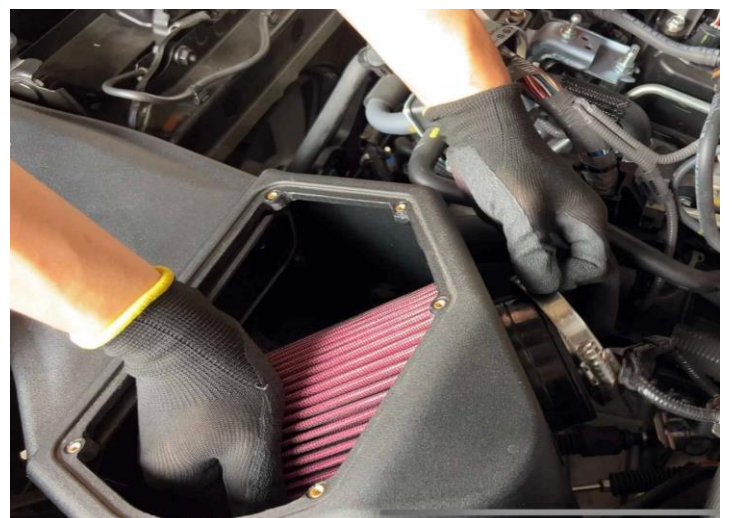
Figure 24: Install the MST filter.
