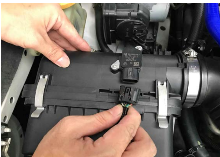
Figure 5: 斷開MAF接頭
