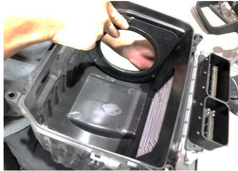
Figure 20: Align MST heatshield.
