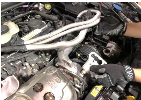
Figure 13: Remove the sensor and the bracket
