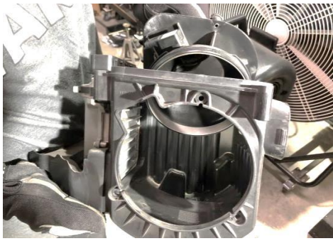
Figure 16: Remove the adapter on the stock air box
