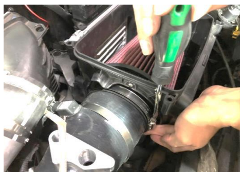
Figure 26: Tighten the clamps between the filter and the hose
