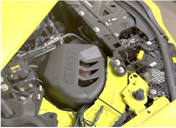
Figure 13: Congratulations! You have just completed the installation of this intake system. Periodically, check the alignment of the intake, normal wear and tear can cause nuts and bolts to come loose.
