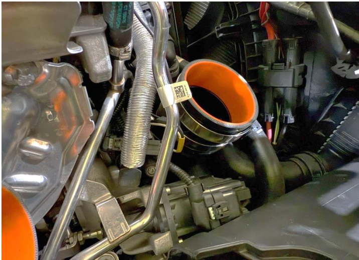
Figure 9: Install silicone hose on the turbo.
