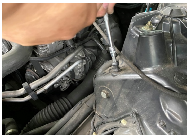
Figure 8: Remove the bolt.拆下螺栓
