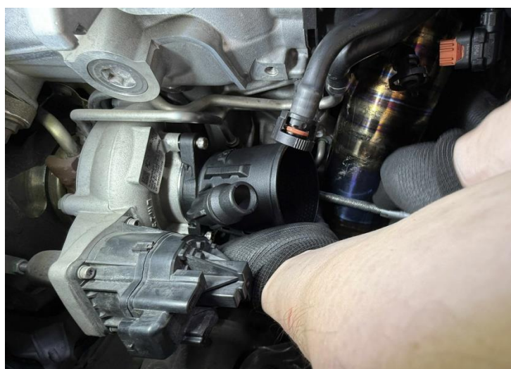
Figure 8: Tighten the bolts. 步驟8: 增流管安裝到渦輪上鎖緊螺絲
