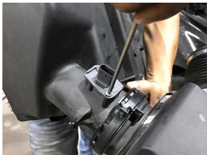
Figure 9: Remove the mass air flow sensor from the stock air box. 從備用集氣箱取出空氣質量流量感應器
