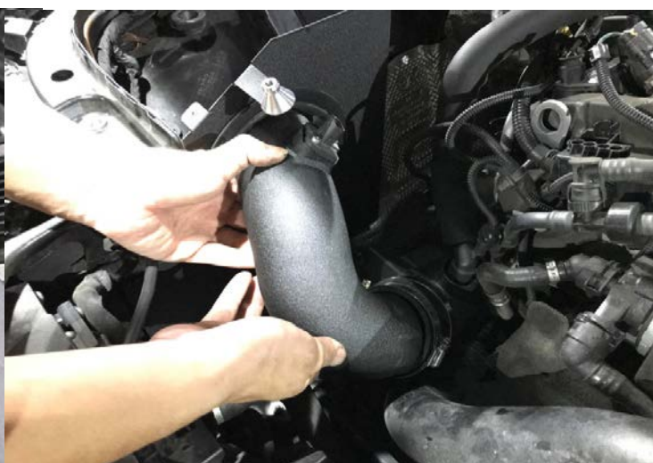
Figure 12: Install mst intake tube.安裝 MST 進氣管
