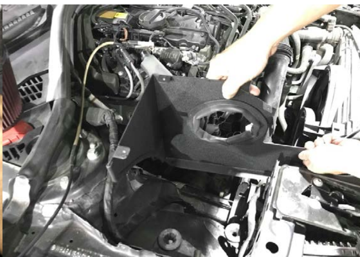
Figure 6: Set the heat shield. 安裝隔熱罩
