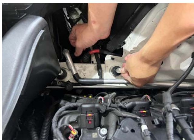
Figure 3: Install the ALU mount and rubber. 安裝 ALU 安裝座和橡膠
