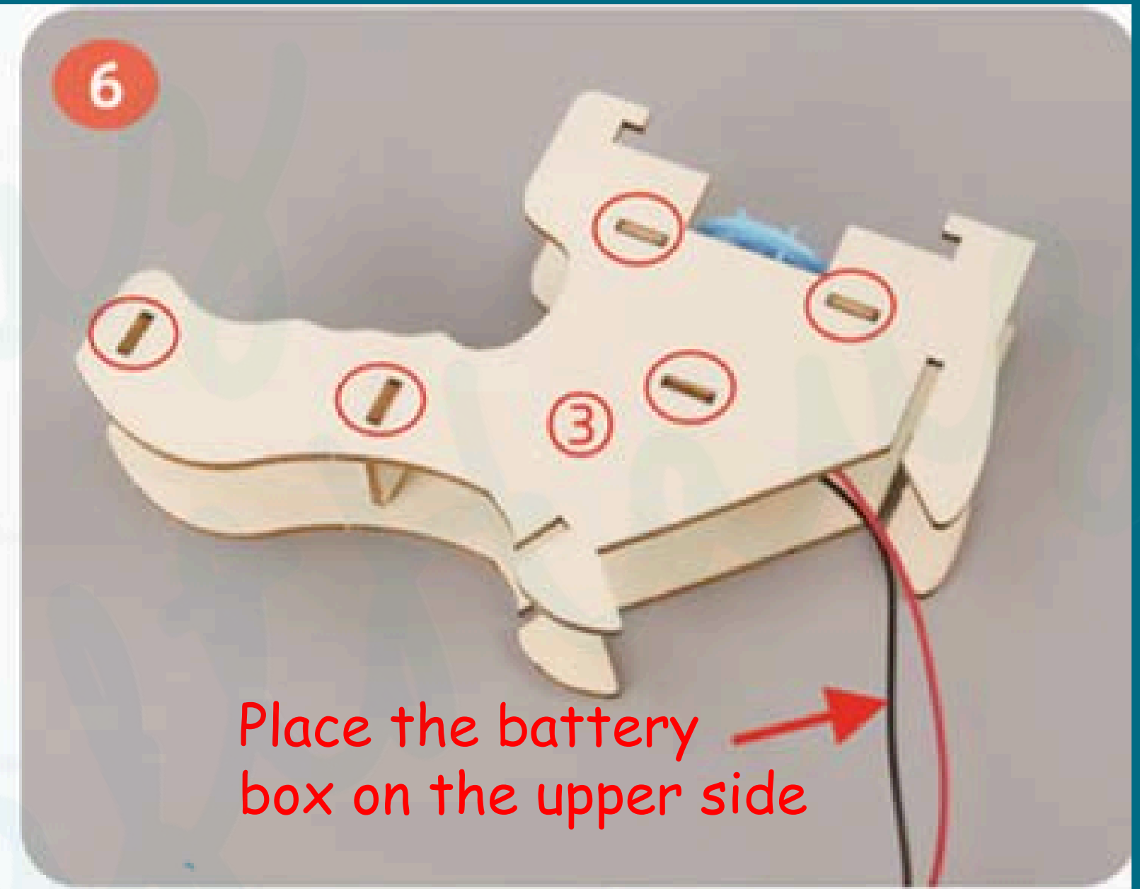
As shown, align the red circle marks and install board 3 side
