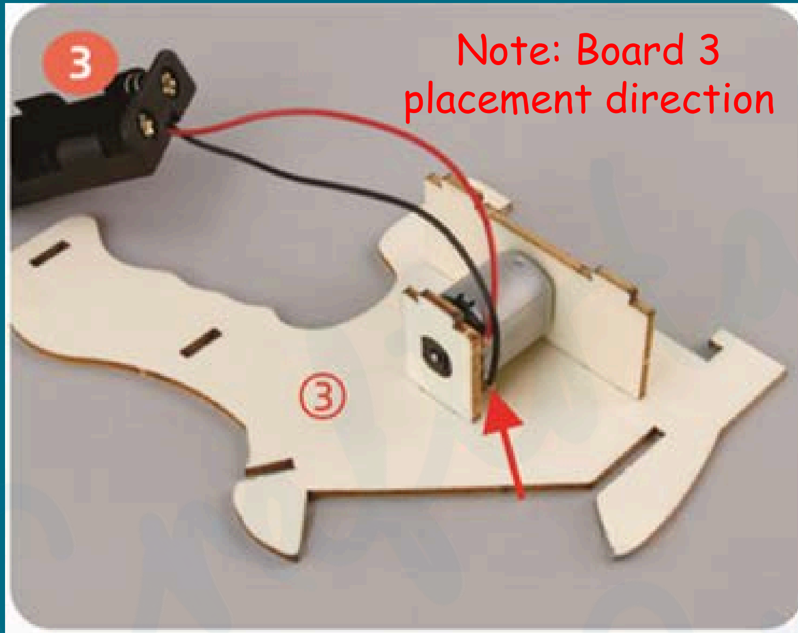
As shown, insert step 2 components into board 3 side
