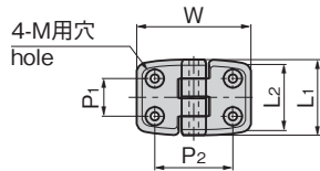
BP-19-1-2-S 皿ねじ用 For countersink screw
